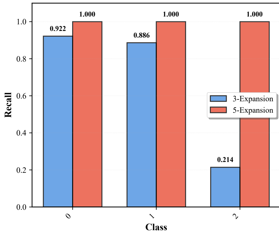
(b) Recall per Class
