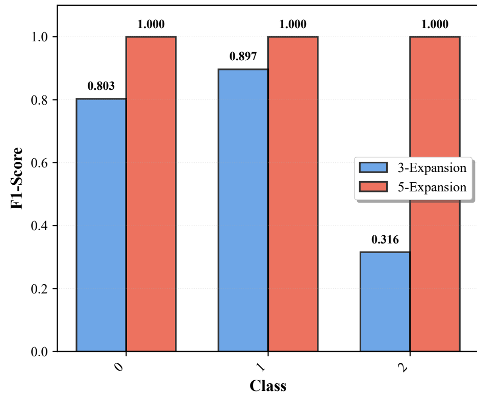
(c) F1-Score per Class
